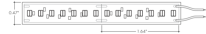
LLWD51WET-WHT-HO (364lm/ft, 4.7W/ft) Max Run Length (in series):22ft
