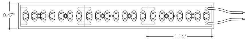
LLVC72WET-WHT-SO (401lm/ft, 3.7W/ft) Max Run Length (in series):28ft
