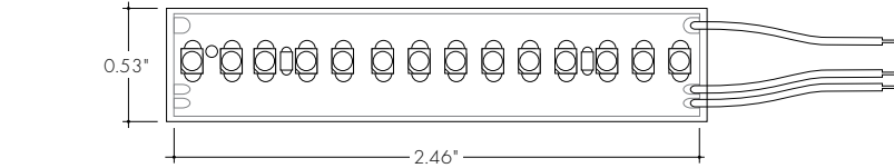
LLTW51WET-WHT-SO (341lm/ft, 4.4W/ft) Max Run Length (in series):29ft
