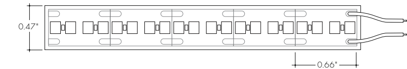
LLVC72WET-WHT-SO (401lm/ft, 3.7W/ft) Max Run Length (in series):28ft
