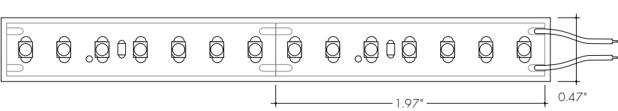
LLHE48WET-T-LO (231lm/ft, 1.9W/ft) Max Run Length (in series):48ft
