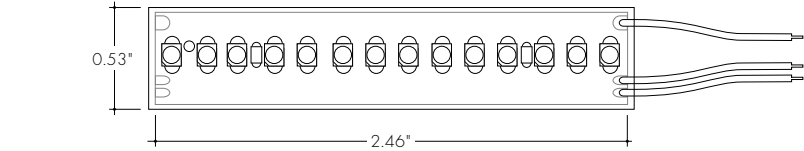
LLTW51WET-WHT-HO (421lm/ft, 5.4W/ft) Max Run Length (in series):22ft
