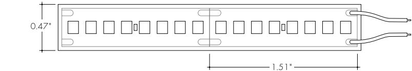
LLHE64WET-WHT-HO (766lm/ft, 5.6W/ft) Max Run Length (in series):17.0ft
