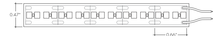
LLVC72WET-WHT-HO (641lm/ft, 6.0W/ft) Max Run Length (in series):21ft
