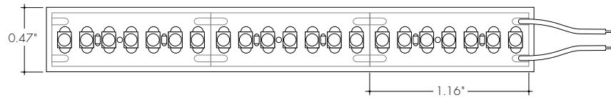
LLVC72WET-WHT-LO (302lm/ft, 2.8W/ft) Max Run Length (in series):32ft
