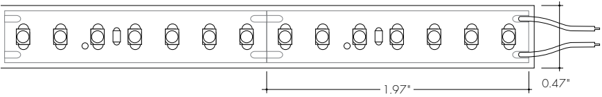
LLVC72WET-WHT-LO (302lm/ft, 2.8W/ft) Max Run Length (in series):32ft
