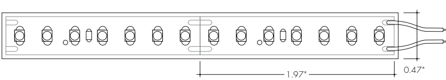
LLHE48WET-T-SO (330lm/ft, 2.8W/ft) Max Run Length (in series):42ft
