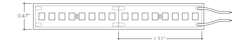
LLHE64WET-WHT-SO (406lm/ft, 2.9W/ft) Max Run Length (in series):34.9ft
