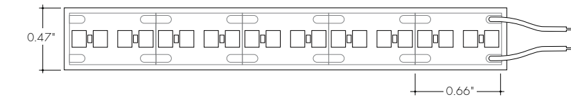
LLVC72WET-WHT-MO (530lm/ft, 4.9W/ft) Max Run Length (in series):24ft
