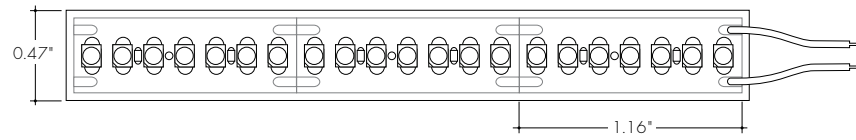
LLVC72WET-WHT-MO (530lm/ft, 4.9W/ft) Max Run Length (in series):24ft
