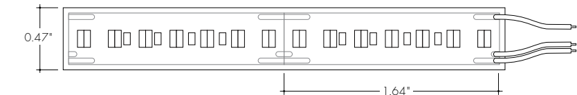
LLTW51WET-WHT-HO (421lm/ft, 5.4W/ft) Max Run Length (in series):22ft
