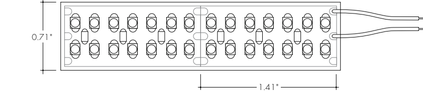
LLVC72WET-WHT-HO (641lm/ft, 6.0W/ft) Max Run Length (in series):21ft
