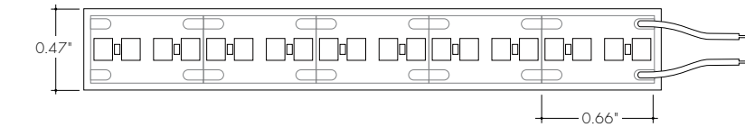
LLVC72WET-WHT-LO (302lm/ft, 2.8W/ft) Max Run Length (in series): 32ft
