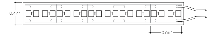
LLVC72WET-WHT-VLO (118lm/ft, 1.1W/ft) Max Run Length (in series):56.9ft
