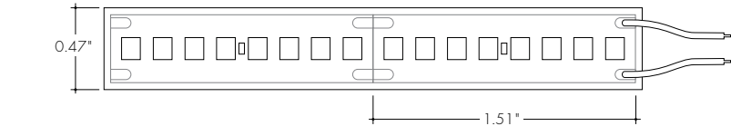
LLHE64WET-WHT-MO (540lm/ft, 3.8W/ft) Max Run Length (in series):25.9ft
