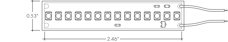
LLWD51WET-WHT-HO (364lm/ft, 4.7W/ft) Max Run Length (in series):22ft
