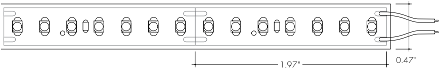
LLVC72WET-WHT-VLO (118lm/ft, 1.1W/ft) Max Run Length (in series):56.9ft
