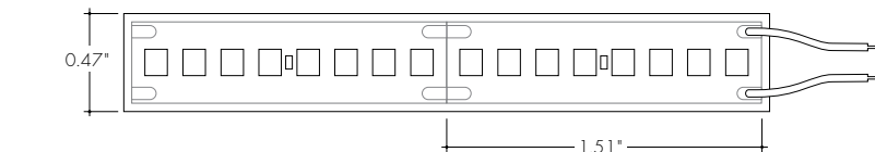
LLHE64WET-WHT-LO (283lm/ft, 1.9W/ft) Max Run Length (in series):55ft
