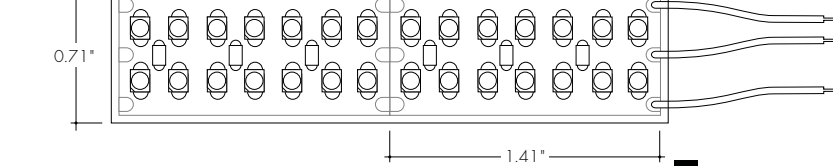
LLTW51WET-WHT-VHO (575lm/ft, 7.6W/ft) Max Run Length (in series):15ft
