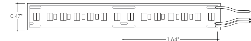
LLTW51WET-WHT-VHO (575lm/ft, 7.6W/ft) Max Run Length (in series):15ft
