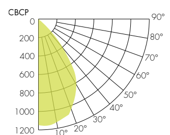
Tunable White 60° Faceted Reflector
