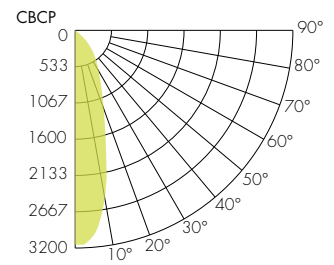
Tunable White 20° Faceted Reflector
