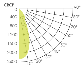
Tunable White 30° Faceted Reflector
