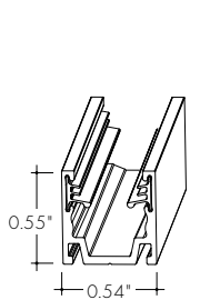
KBS Mounting Channel, Serrated Aluminum Profile
