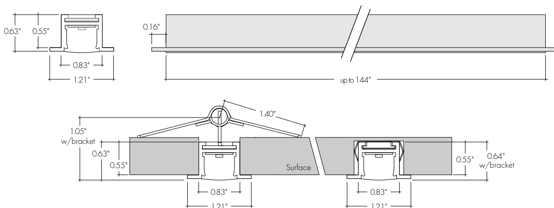
GS - Gypsum surface mounting bracket
