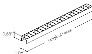
LV-GS-BARC-24-XX Glare Shield reduces glare at high angle, field cuttable. Also available with complete fixture, use ordering code
