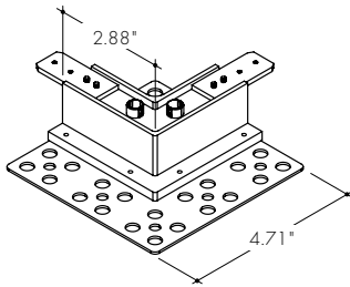
JOIN-M-L-STD-FF-XX Recessed Deep Trimless Mechanical L Joiner
