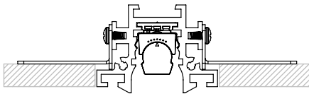
Stenos Deep Trimless Track with Directional Module and Louver
