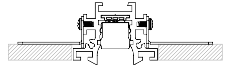
Stenos Deep Trimless Track with Ambient Module and Louver
