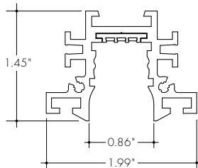
STD-48/95/144-FF/MF-XX Stenos Deep Trimless Track, Recessed
