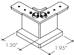
For creating a 90° in-plane corner For use with MF Backer Flange only.
