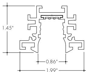
STD-48/95/144-FF/MF-XX Stenos Deep Trimless Track, Recessed
