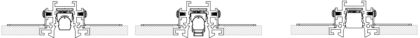
Stenos Deep Trimless Track with Directional Module and Louver
