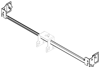
For use to mount to joists. MB-STL not included.
