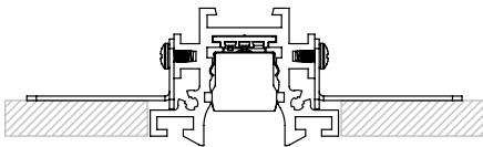
Stenos Deep Trimless Track with Ambient Module and Louver
