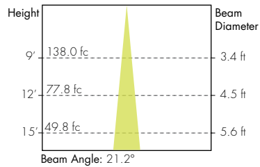
30° Faceted Reflector
