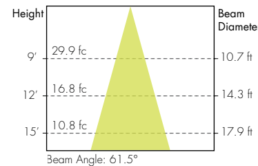
60° Faceted Reflector
