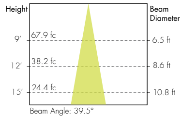
45° Faceted Reflector
