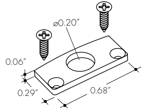
EC-BSC-H1-SA Silver Anodized End Cap with powerfeed opening
