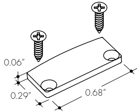
EC-BSC-H0-SA Silver Anodized End Cap
