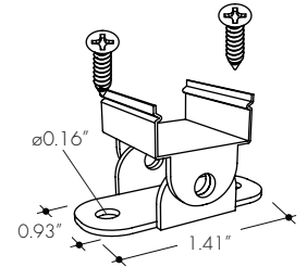
MB-BMSC-A-SS Adjustable Clip -A
