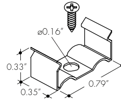
MB-BMSC-SS Fixed Clip -FC
