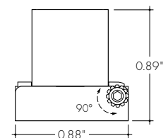
Adjustable Bracket
