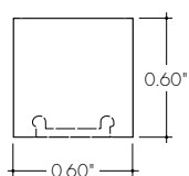
Fixed Clip
