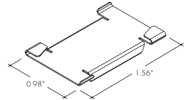
MB-BARC-TB15-SS Bara 15/16" Lay-in Grid Mounting Bracket -TB15
