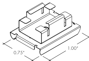
MB-BARC-TT9-SS Bara 9/16" Tegalur Mounting Bracket -TT9
