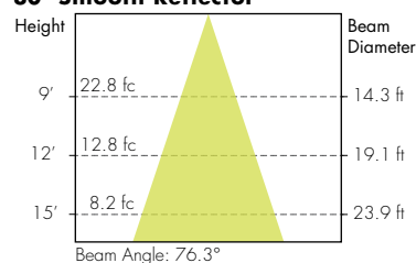
80° Smooth Reflector
