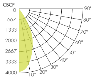
80° Smooth Reflector
