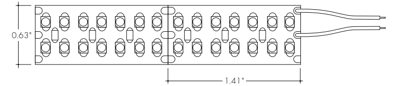
LL60X2-HO
