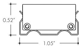
BLC with Fixed Clip
