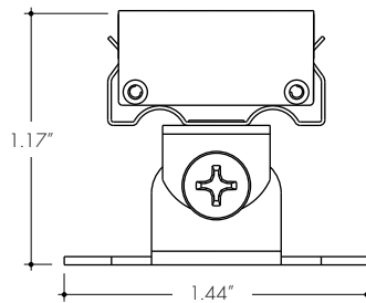
BLC with Adjustable Clip
