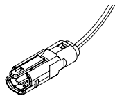
60-H-0001-08 Female Quick Connect with flying leads
