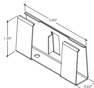
75-CLP19-001-00 Surface Mount, Standard Joiner Clip
