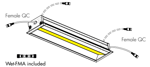
4 Dual Female Quick Connect
