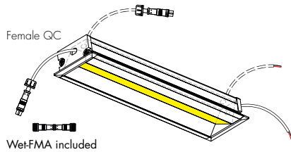
2 72" wire leads at selected end and Female Quick Connect at other
