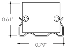
BMC with Fixed Clip
